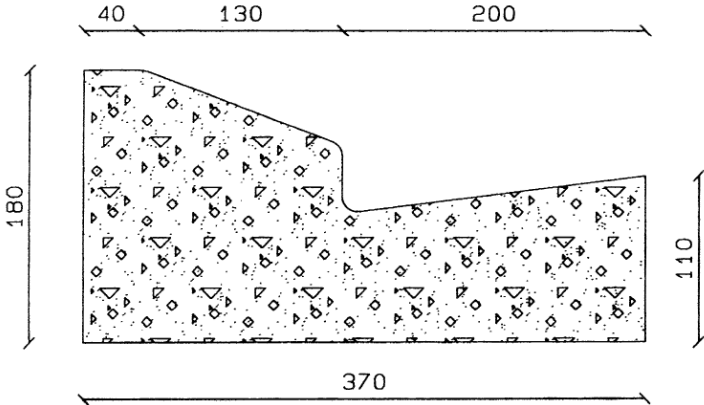
ROLL-OVER (PARROW/CK 5)
