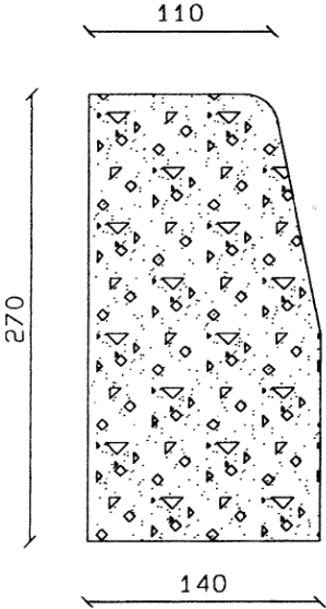
BARRIER (BK 1)
